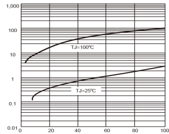
FIG. 4-TYPICAL REVERSE CHARACTERISTICS
